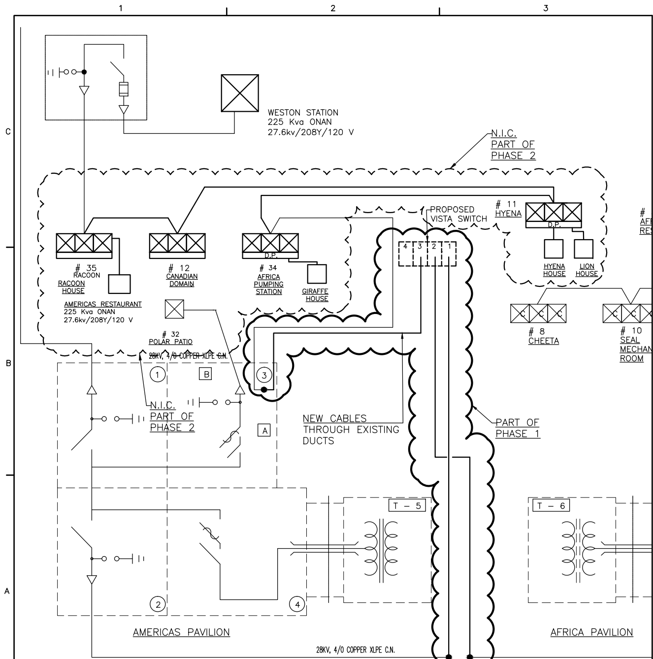
1 PART DWG. E-02 Scale: NO SCALE
